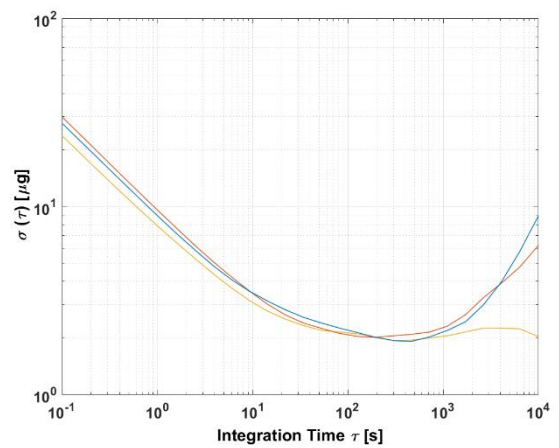
Figure 24: Allan Variance
