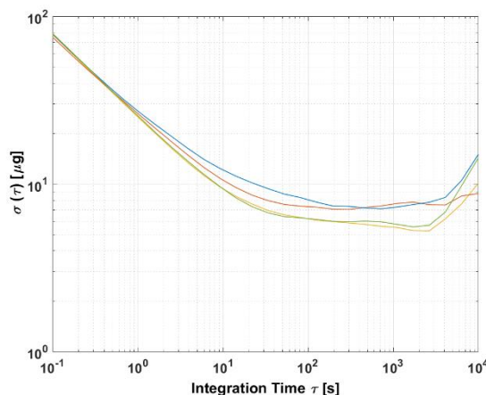
Figure 34: Allan Variance
