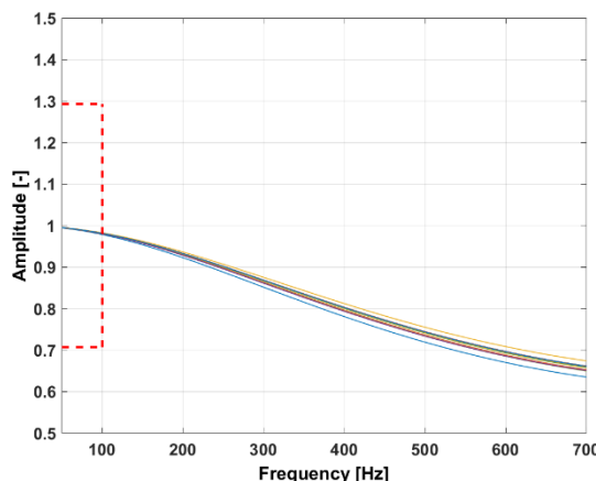
Figure 32 : Frequency response
