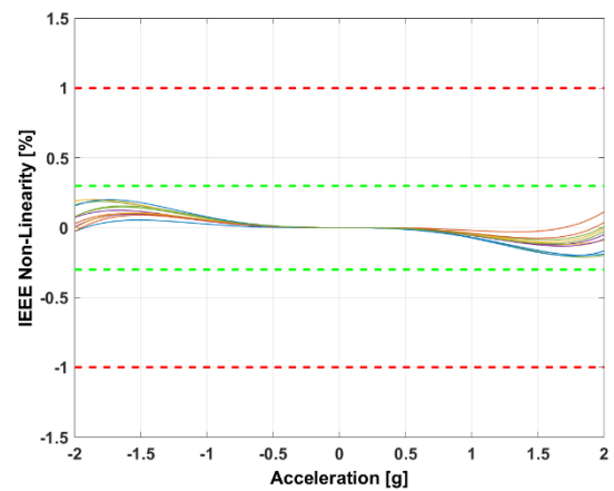
Figure 10 : Non-linearity IEEE
