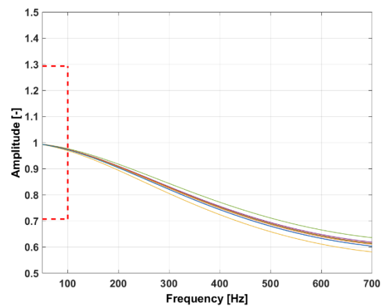
Figure 12 : Frequency response
