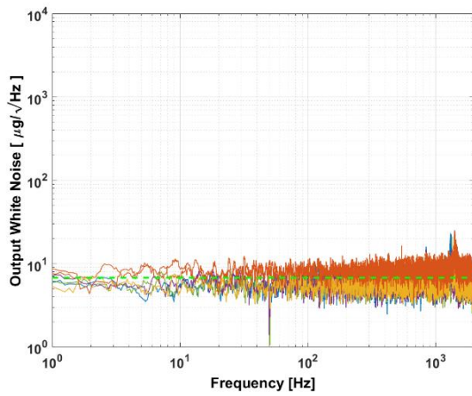
Figure 13: Typical white noise
