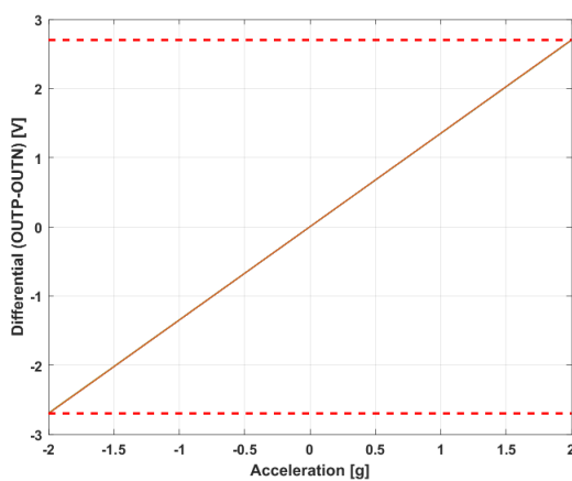
Figure 11 : Differential acceleration output (OUTP-OUTN) at full scale
