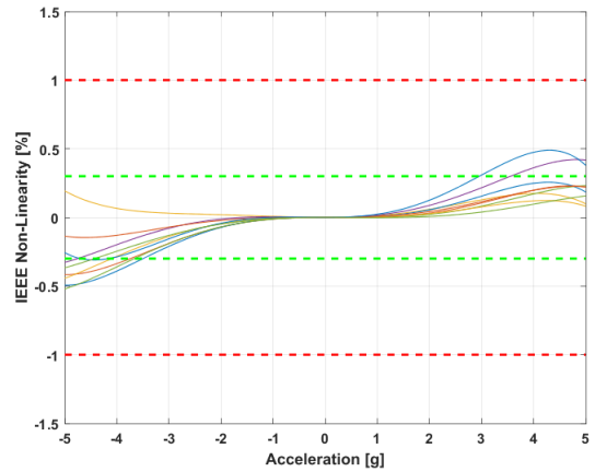
Figure 20 : Non-linearity IEEE
