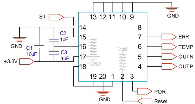
Figure 36: Proximity circuit & internal pull-up/down
