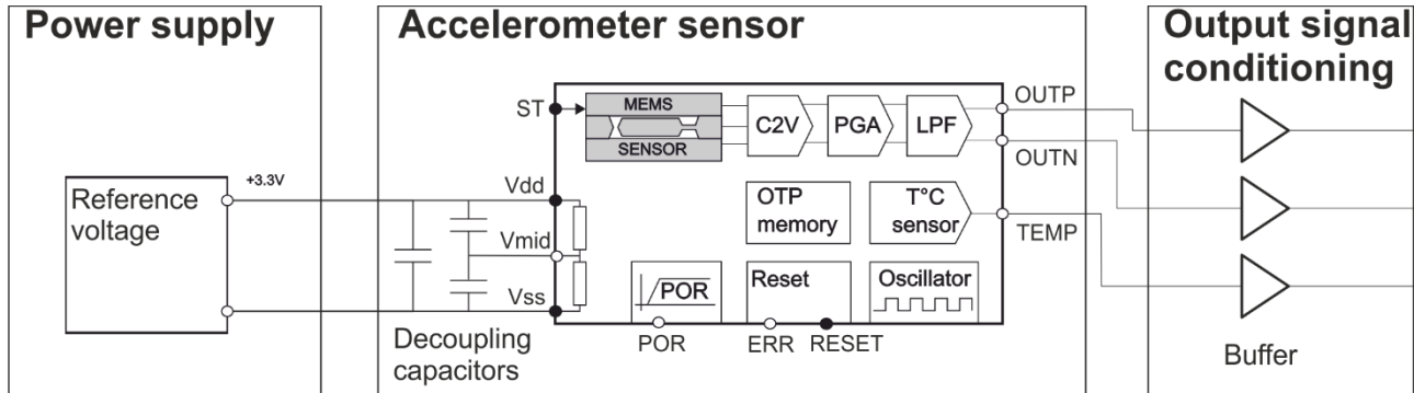
Figure 42: Block diagram
