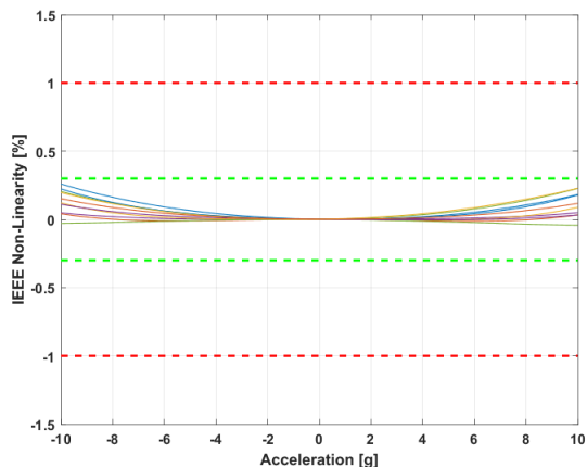
Figure 30 : Non-linearity IEEE
