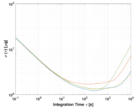
Figure 14: Allan Variance
