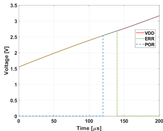
Figure 15: Typical sensor power sequence using recommended circuit
