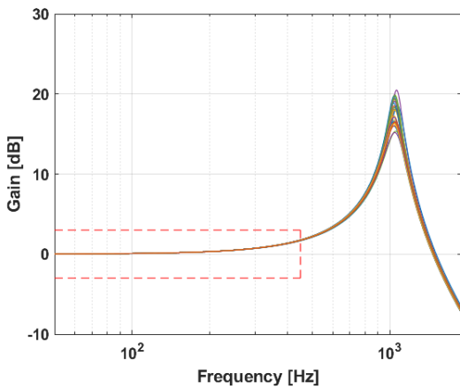
Figure 3: Frequency response
