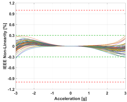
Figure 2: Non-Linearity IEEE
