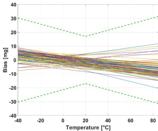
Figure 11: Bias over temperature
