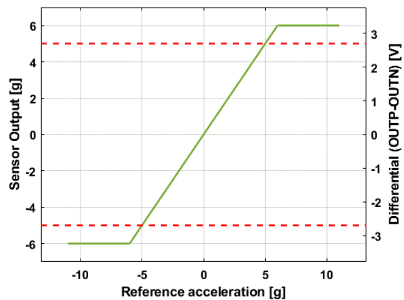
Figure 21: SI1005 versus reference sensor
