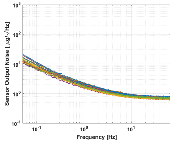
Figure 4: Noise Spectrum
