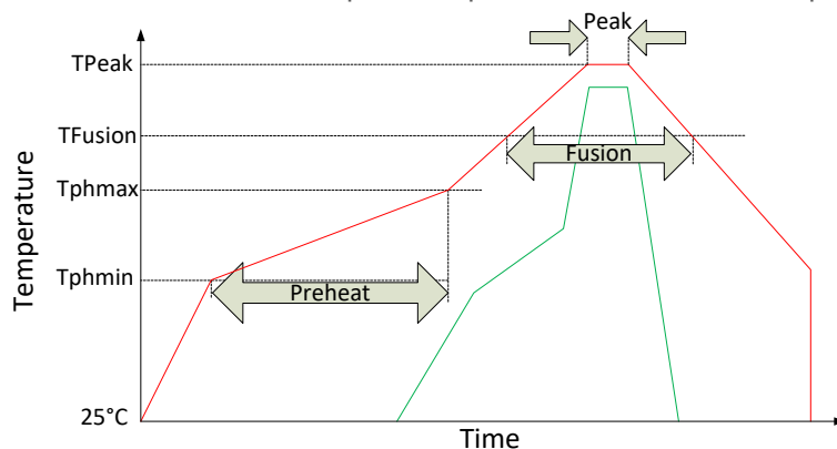
Figure 25: Soldering Temperature Profile
