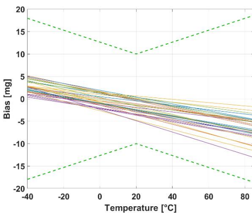
Figure 5: Bias over temperature
