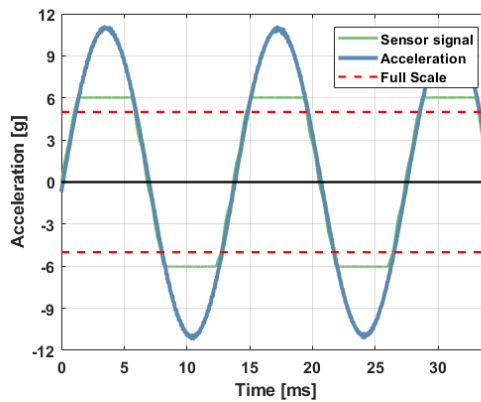
Figure 19: 5g Sensor response to 11g sine
