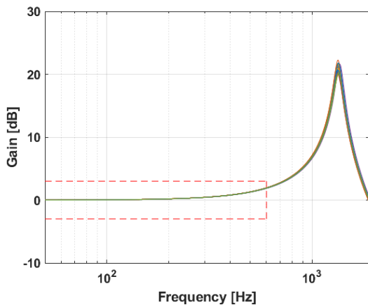
Figure 9: Frequency response
