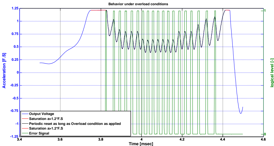
Figure 42 : Overload Behavior
