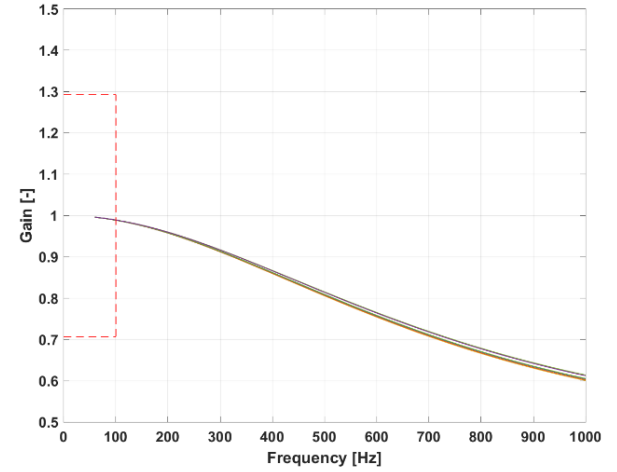
Figure 16 : Frequency response
