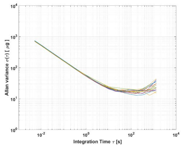
Figure 24: Allan Variance
