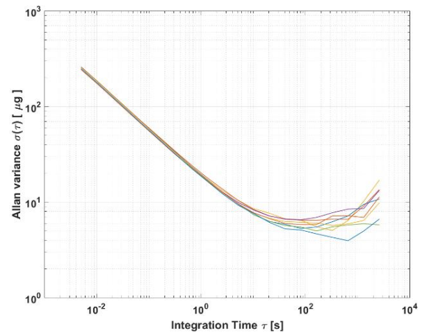
Figure 18: Allan Variance
