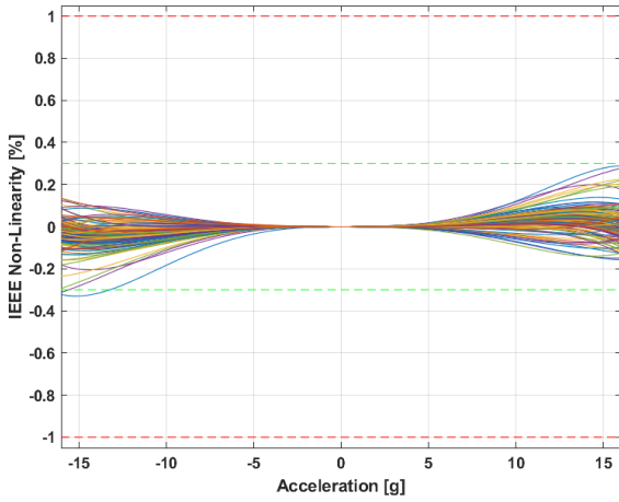
Figure 42 : Non-linearity IEEE
