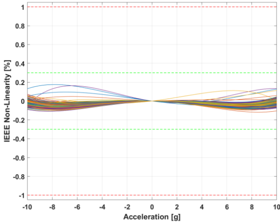
Figure 31 : Non-linearity IEEE
