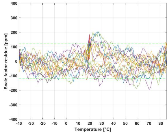
Figure 51: Residual Scale Factor over temperature
