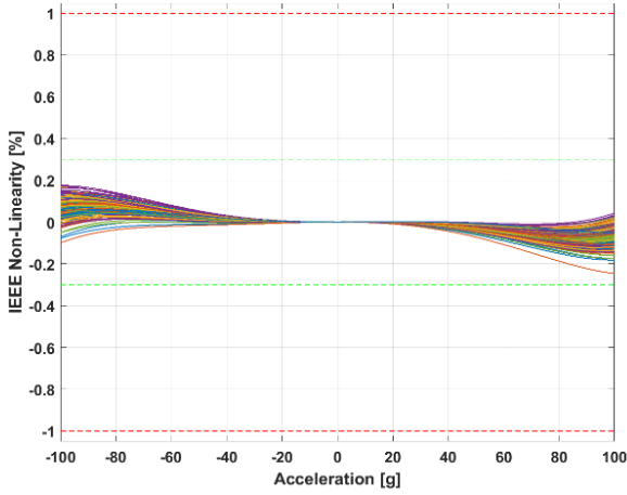
Figure 66 : Non-linearity IEEE
