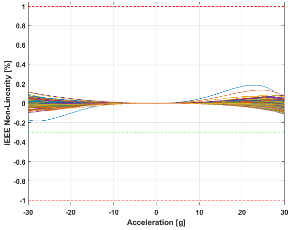
Figure 54 : Non-linearity IEEE
