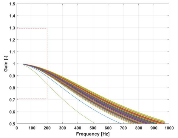
Figure 33 : Frequency response
