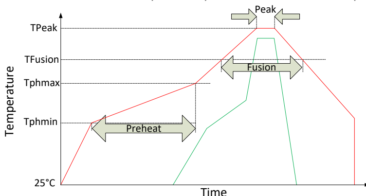
Figure 81: Soldering Temperature Profile
