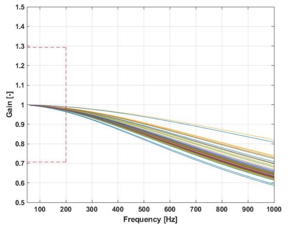
Figure 45 : Frequency response
