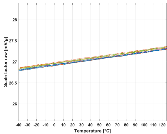
Figure 65: Raw scale factor over [-55°C to +125°C]
