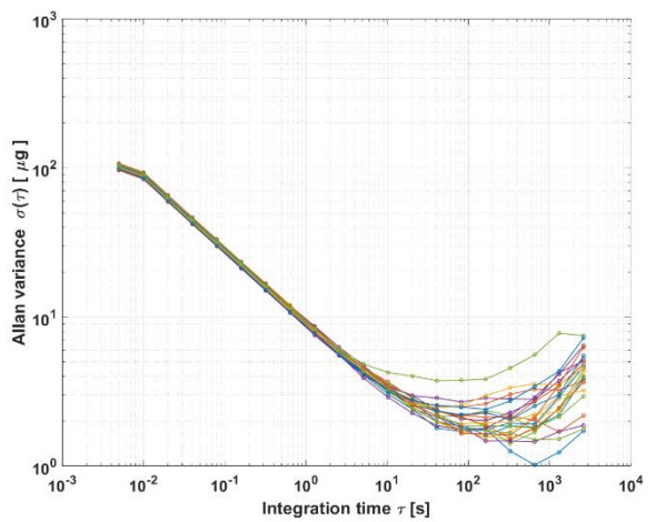
Figure 24: Allan Variance
