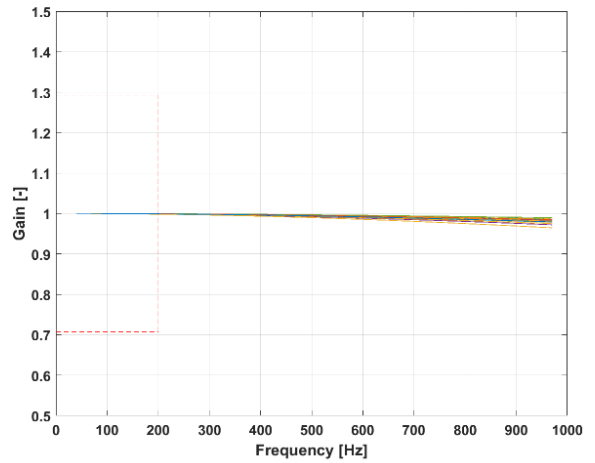
Figure 69 : Frequency response
