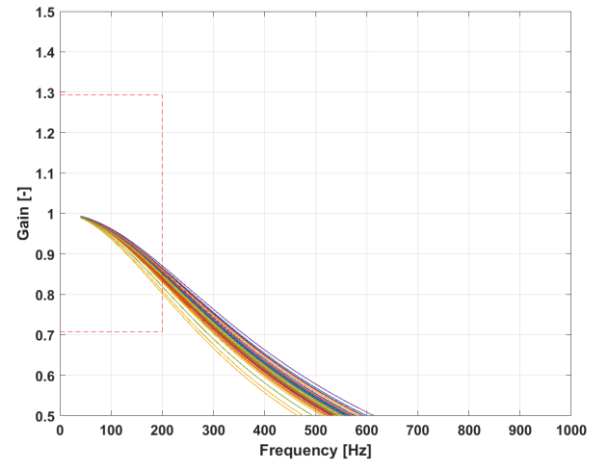
Figure 10 : Frequency response
